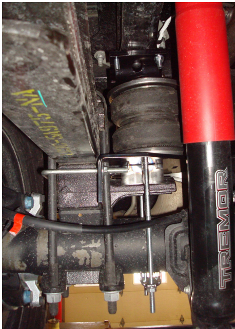
Passenger's (right) side front view
