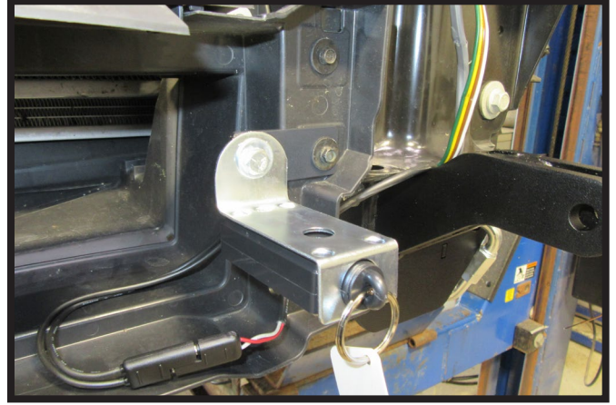
25. Optional Breakaway: Install breakaway bracket to vehicle using existing bolt. Then install breakaway switch to bracket using provided 1/4" bolt with flat washer and nylon insert lock nut.
