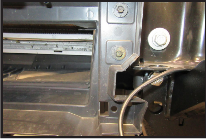
24. Optional Breakaway: Using a 7MM socket, remove the bottom bolt on the driver side of the vehicle.
