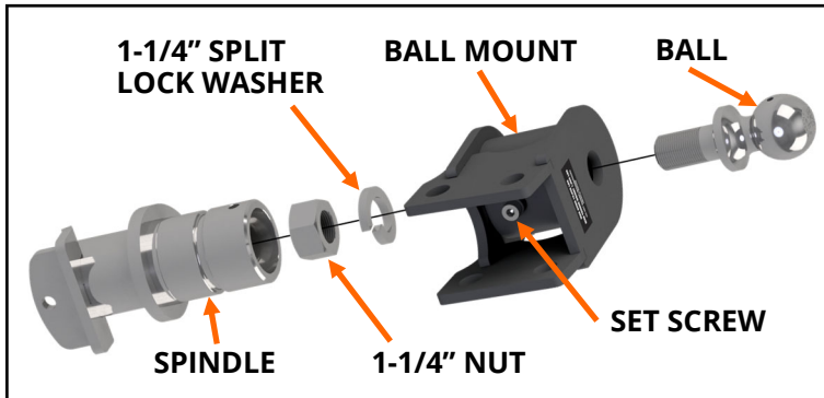
FIGURE K1: View of exploded ball mount.
