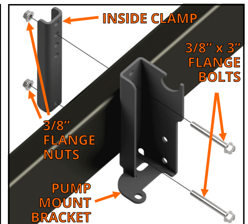
FIGURE C4: View of driver side frame rail.
