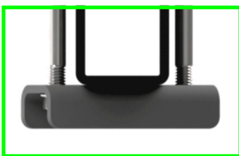
FIGURE D6: View showing a correctly tightened frame clamp.
