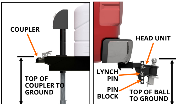
FIGURE B1: Side view of trailer. FIGURE B2: Side view of tow vehicle.
