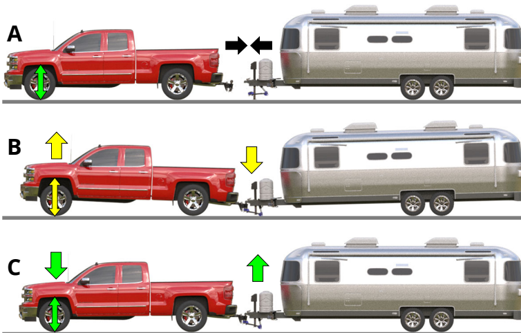
FIGURE H1: View of tow vehicle and trailer showing measurement locations.
